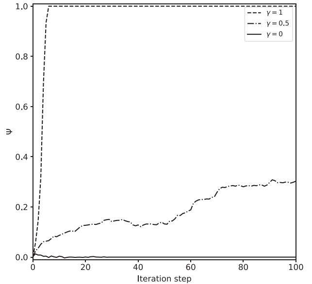
Fig. 1. Three example runs over time, for three parameters of \gamma . \psi is measured every 5,000 steps, over 500,000 time steps. Parameters are b = 8 , n = 10 , |A| = 196 , c = 4 , m = 10 . As the figure shows, the run with \gamma = 1 quickly reaches a high \psi -value. The medium- \gamma population gradually increases to a \psi of 0.3. The run with completely local interaction remains near the expected \psi value of 0.
