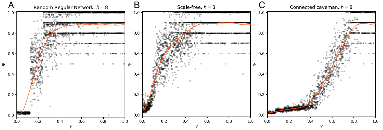
Fig. 3. The model applied on three common network structures, running with otherwise the same parameters as for Fig. 2C, with 1,600 runs over the parameter space. (A) A random regular graph, generated through the algorithm described in Steger and Wormald (112). Parameters used were 196 nodes and 8 edges. (B) A scale-free network, characterized by highly uneven degree distribution with some dominant nodes, generated with the algorithm described in ref. 113, based on Barabási-Albert growth model but adding that each random edge is followed by a chance of making an edge to one of its neighbors, thus capturing clustering. Parameters used were 196 nodes, 8 edges, and 0.01 probability of adding a triangle to any given edge. (C) The connected caveman, a highly cliqued graph structure used also in DellaPosta et al. (58), with 14 cliques of 14 nodes and 0.05 probability for reconnecting a given edge. As can be seen, strikingly, all network structures show the same general relationship between \gamma and \psi but with differences in the immediacy of the rise of sorting as a function of nonlocal interactions. In particular, the clique-dominated network in C requires a higher value of \gamma to become sorted.
